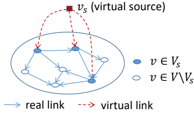
Fig. 2. Auxiliary graph G^0 that augments G by adding a virtual source v_s connected to all real sources in V_s .
