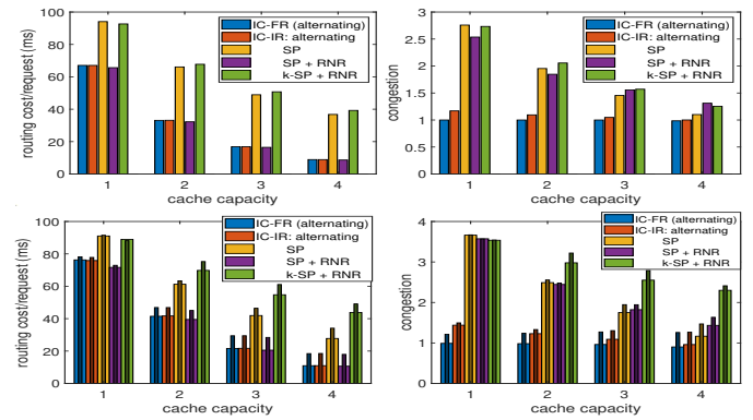
Fig. 7. General case under varying cache capacity: first row – synthetic simulation, second row – trace-driven simulation (light: true demand; dark: predicted demand).
