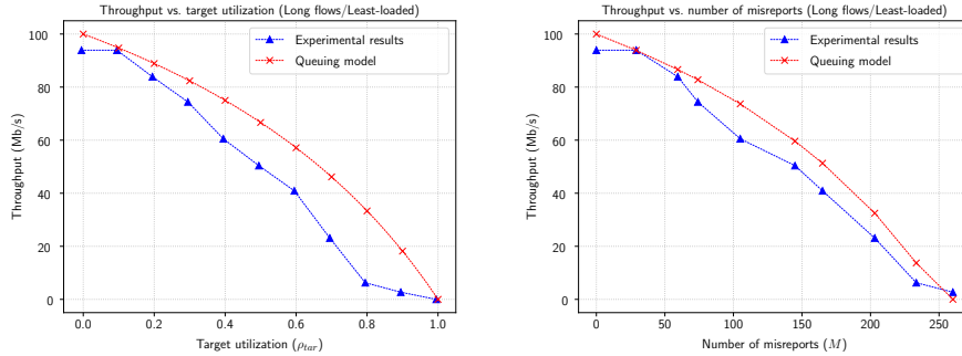
Fig. 4. Throughput vs. target utilization ( \rho_{tar} ) and number of misreports.
